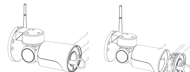
1. Bolts ,2 ,Front cover 3. case ,4.tool
